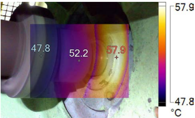
IR005130.IS2-No2 Jacket water pump 12/3/2016 8:54:55 AM
