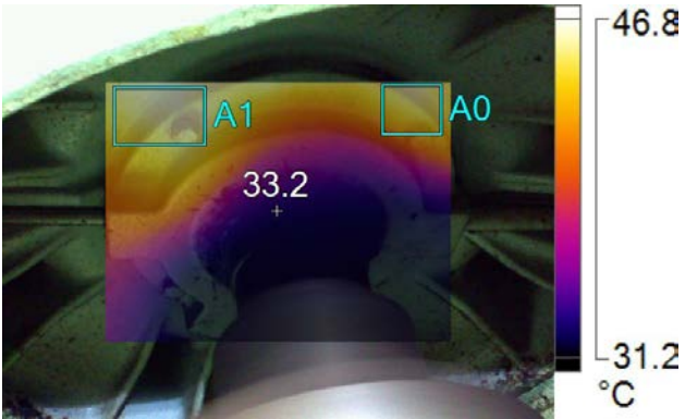
IR005193.IS2-Vac Cond pump
