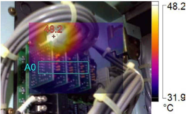
IR005206.IS2-No2 SW Serv pump 12/3/2016 1:26:36 PM
