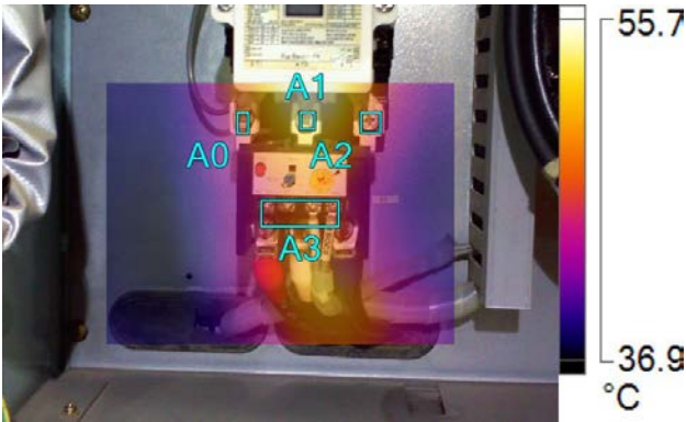
IR005169.IS2-Scrubber Pump 12/3/2016 11:16:50 AM
