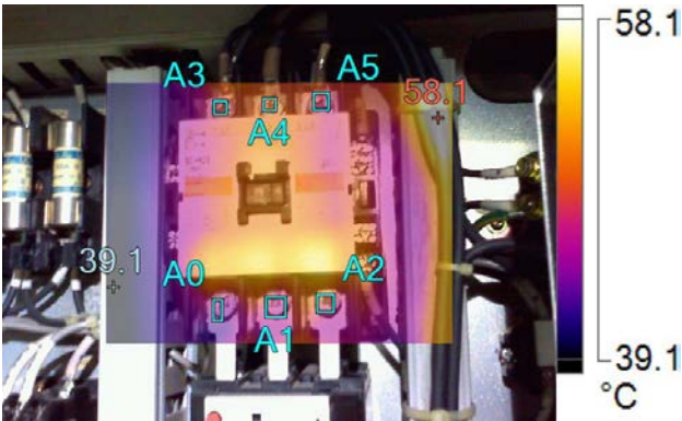
IR005203.IS2-No2 SW Serv pump 12/3/2016 1:24:35 PM
