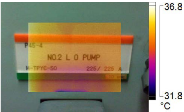
IR005148.IS2-No2 Main LO pump 12/3/2016 9:46:21 AM
