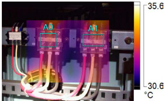
IR005123.IS2-No2 Jacket water pump 12/3/2016 8:52:39 AM
