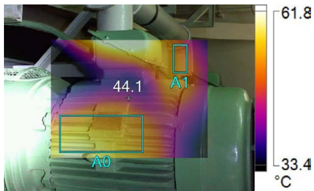
IR005128.IS2-No2 Jacket water pump 12/3/2016 8:54:13 AM
