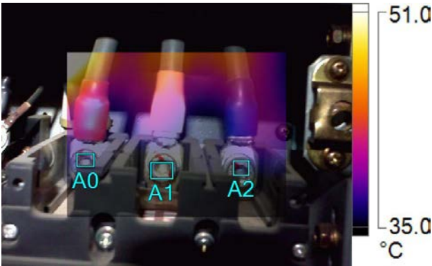
IR005135.IS2- No2 Cooling SW pump
