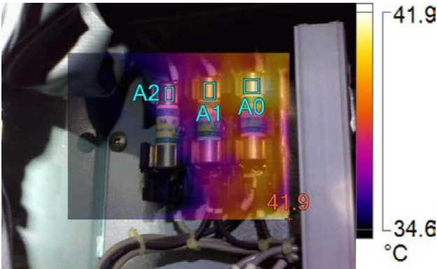
IR005205.IS2-No2 SW Serv pump 12/3/2016 1:24:53 PM
