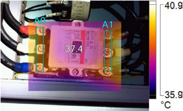
IR005117.IS2- No1 Aux Blower panel
