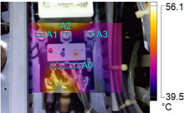
IR005138.IS2- No2 Cooling SW pump
