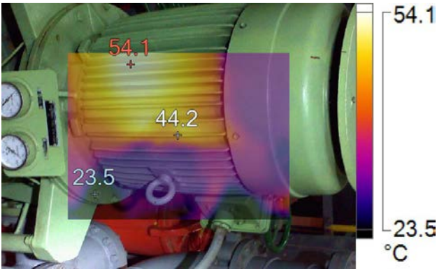
IR005175.IS2-Scrubber Pump 12/3/2016 11:19:14 AM
