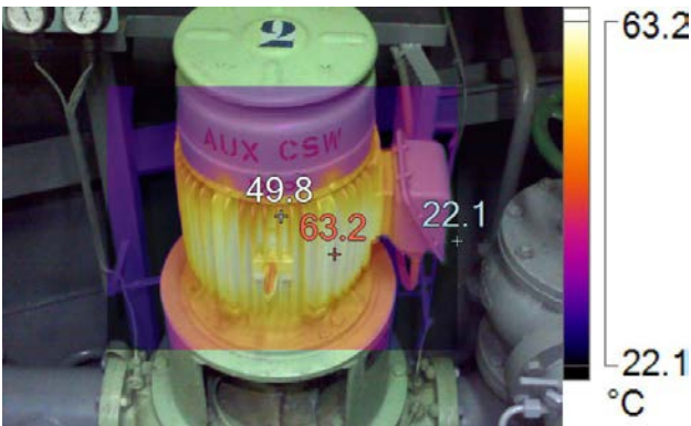
IR005226.IS2- No2 Aux CSW Pump 12/3/2016 1:39:36 PM
