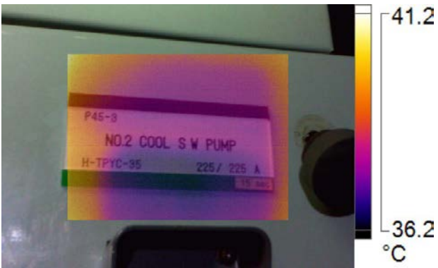
IR005133.IS2- No2 Cooling SW pump 12/3/2016 9:15:53 AM
