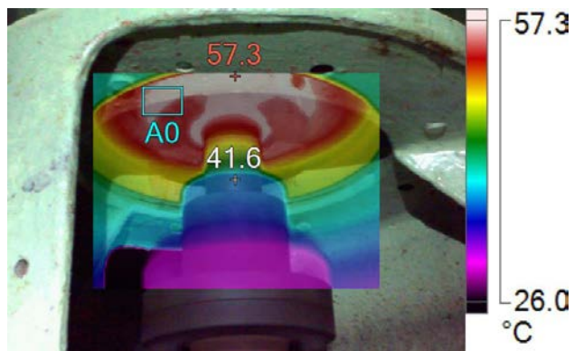
IR005229.IS2- No2 Aux CSW Pump 12/3/2016 1:42:16 PM
