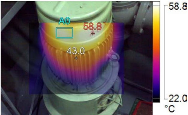
IR005214.IS2-Air Cond SW pump
