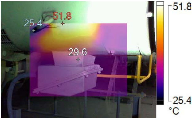
IR005189.IS2-Vac Cond pump
