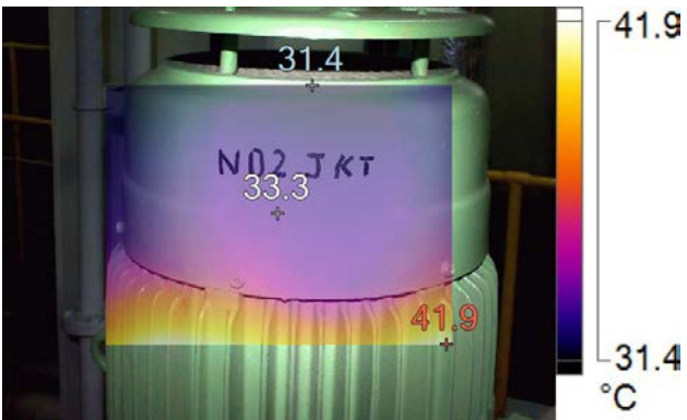
IR005124.IS2-No2 Jacket water pump 12/3/2016 8:53:26 AM
