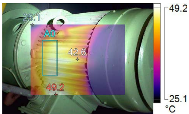
IR005142.IS2-No2 CSW pump
