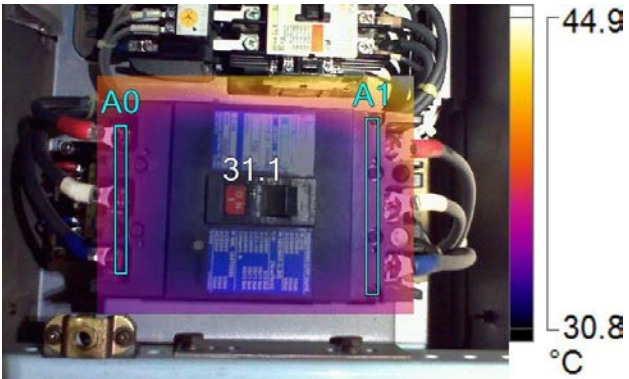
IR005119.IS2-No2 Jacket water pump 12/3/2016 8:51:32 AM
