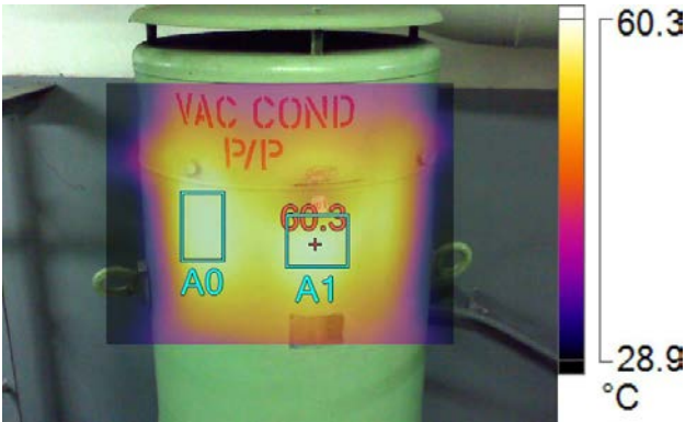
IR005186.IS2-Vac Cond pump 12/3/2016 11:50:45 AM
