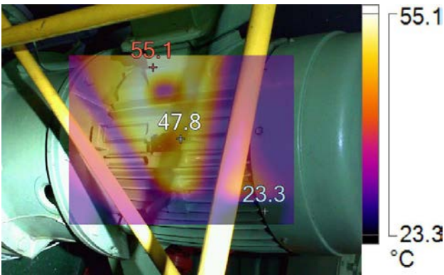
IR005174.IS2-Scrubber Pump 12/3/2016 11:18:45 AM
