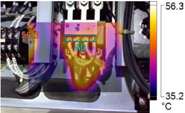
IR005204.IS2-No2 SW Serv pump 12/3/2016 1:24:42 PM
