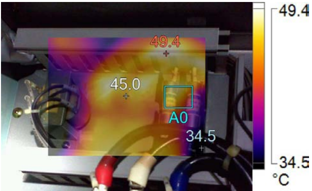
IR005184.IS2-Cargo Cond Circ pump 12/3/2016 11:48:09 AM
