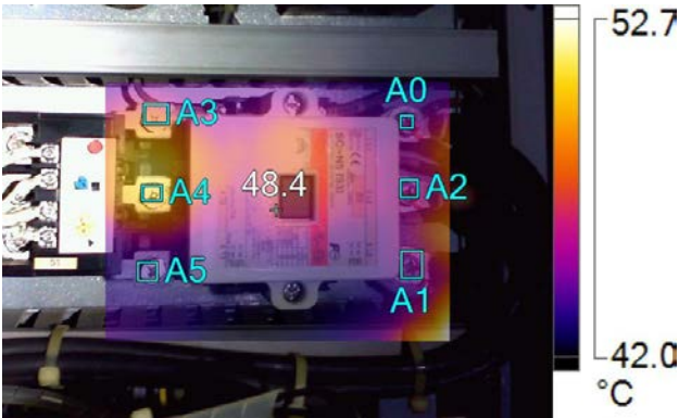
IR005137.IS2- No2 Cooling SW pump
