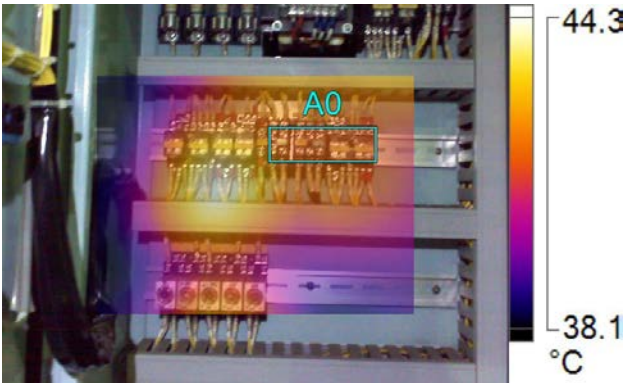
IR005114.IS2- No1 Aux Blower panel
